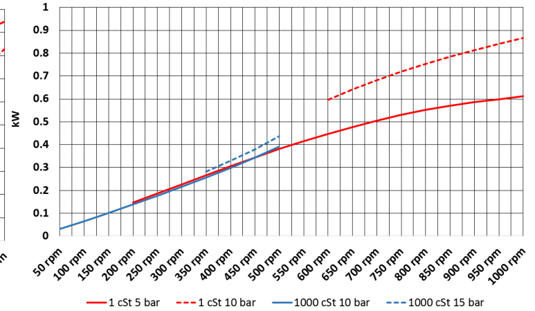
Absorbed power
