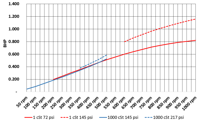
Absorbed power
