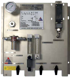
Stainless Steel Gas Panel Image 2
