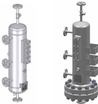
AES-28™ Vessel with Socket Welded Flanges (Left) AES-28-FV™ utilises a bottom flange that can be removed to administer efficient internal cleaning (Right)
