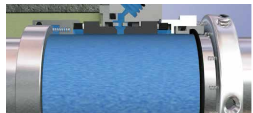
4. Double mechanical seal with cool / clean barrier fluid
