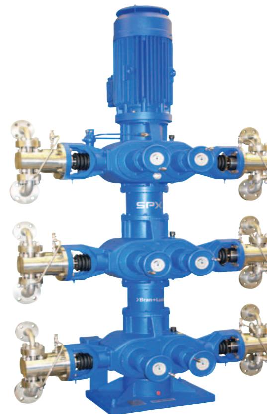
Vertical metering pump with multiple plunger pump heads
