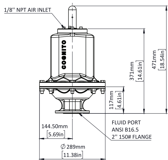
Stainless Steel Dampener Model: 2SXU
