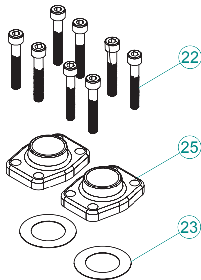
Flange set for welding
