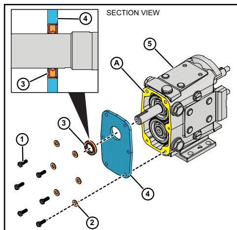
Figure 71 - Install Cover Lip Seal and Cover
