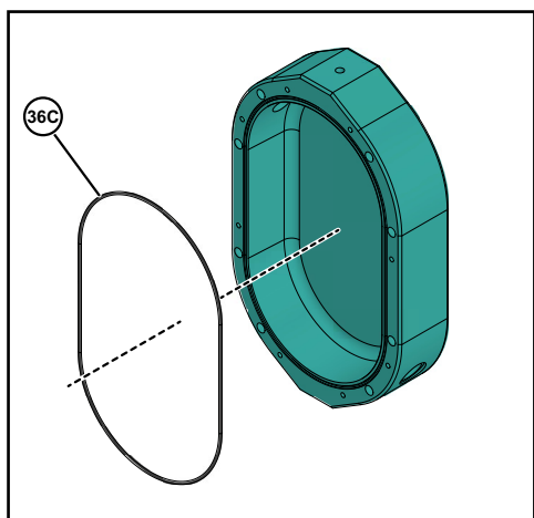
Figure 110 - Install Gasket
