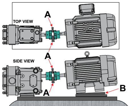
Figure 23 - Check Angular Alignment
