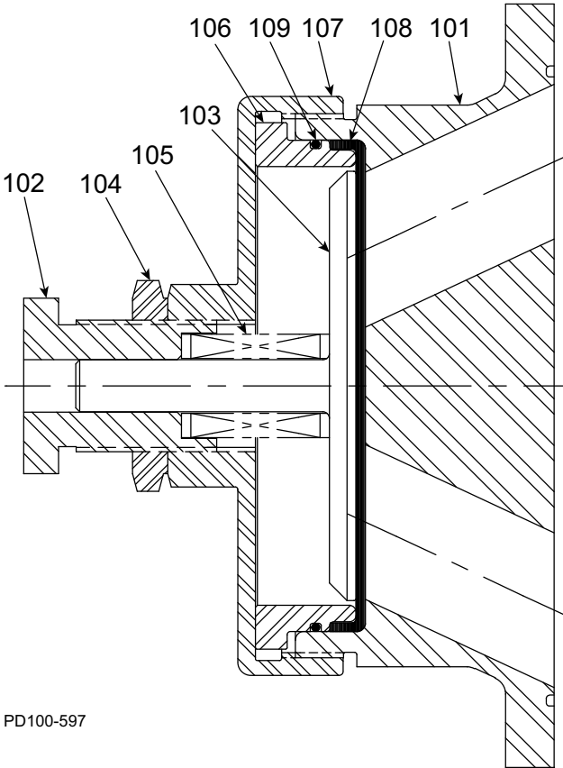
Figure 130 - Manual Vented Cover, 180-220-224 U2
