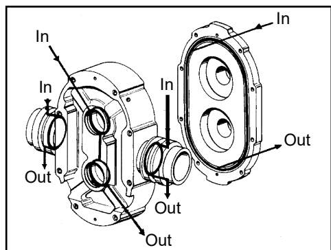
Figure 112 - Flushing Connection - Aseptic Series
