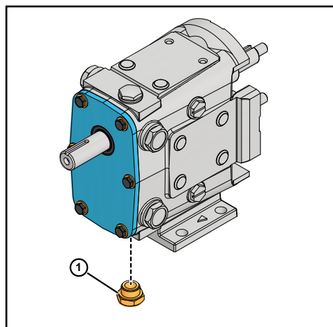
Figure 72 - Install Oil drain Plug
