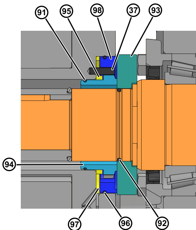
Figure 123 - Standard Double Mechanical Seal
