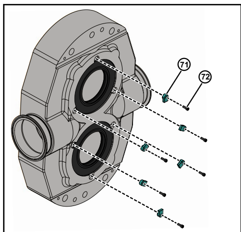
Figure 114 - Remove Screws and Retainer-tab
