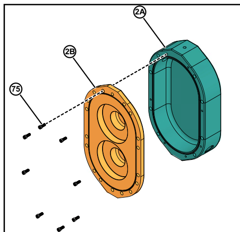
Figure 111 - Attach cover and jacketed cover
