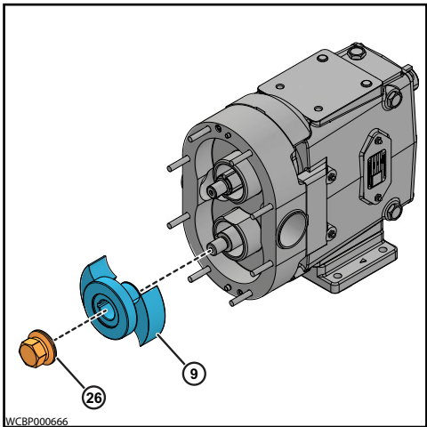
Figure 80 - Install Rotor and Nut
