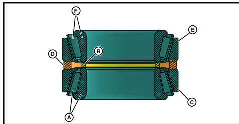
Figure 52 - Bearing assembly
