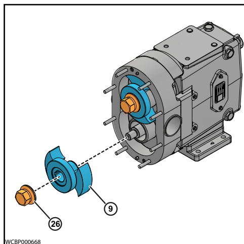
Figure 82 - Install Rotor and Nut
