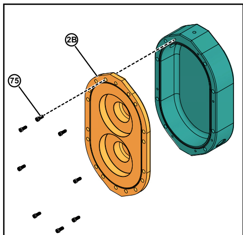
Figure 109 - Remove Gasket
