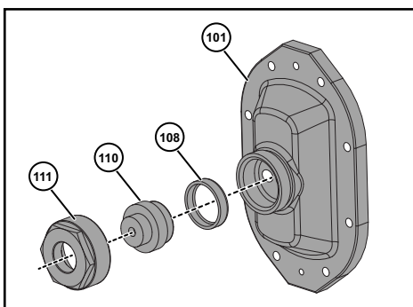
Figure 85 - Pneumatic Diaphragm Cover
