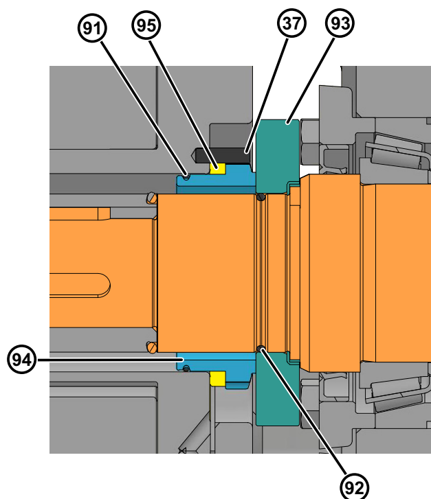
Figure 122 - Standard Single Mechanical Seal
