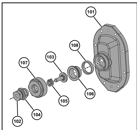
Figure 84 - Manual Cover
