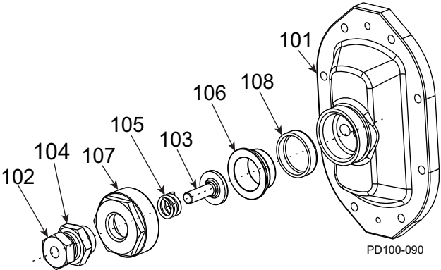
Figure 128 - Manual Vented Cover, 006-134-U2
