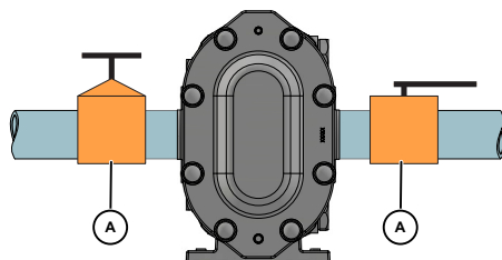
Figure 13 - Isolation Valves
