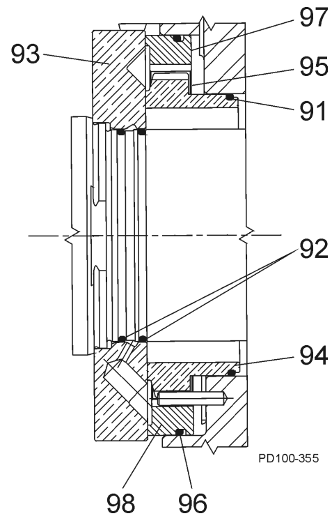
Figure 124 - Aseptic Design Double Mechanical Seal (213, 323 U2 ONLY)
