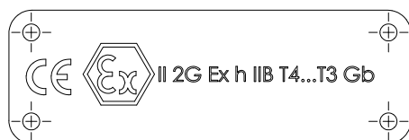
Figure 133 - ATEX Nameplates
