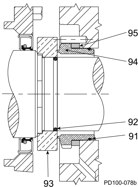
Figure 125 - NF Single Mechanical Seal
