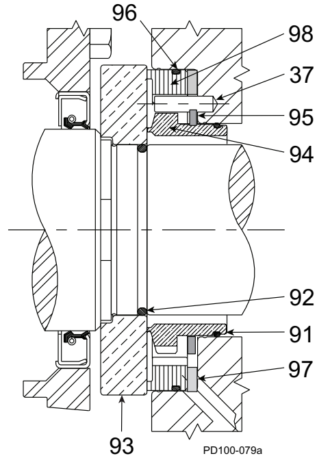
Figure 126 - NF Double Mechanical Seal
