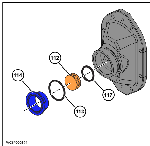
Figure 102 - Remove Diaphragm Bushing
