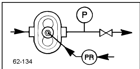
Figure 106 - Adjustment with a Pressure Gauge
