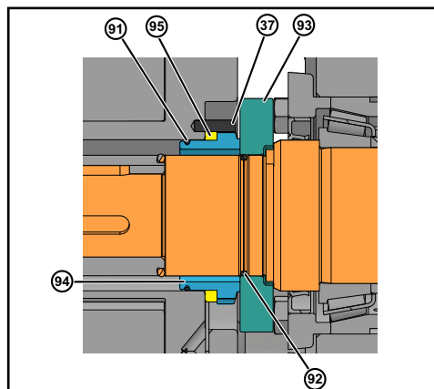
Figure 74 - Single Mechanical Seal
