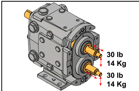
Figure 31 - Bearing Deflection Check
