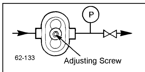
Figure 105 - Manual Adjustment
