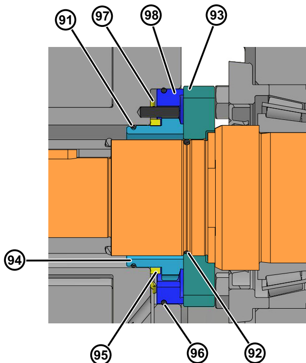
Figure 127 - High Pressure Barrier (HPB) Seal
