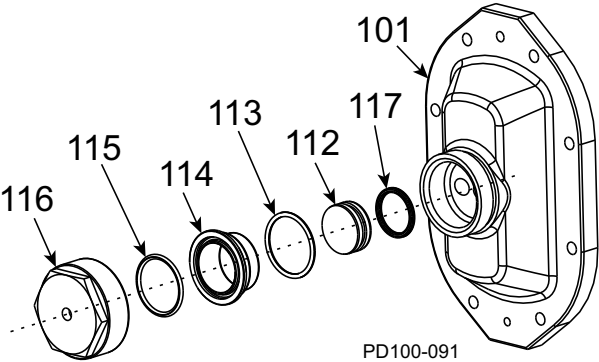
Figure 131 - Pneumatic Piston Vented Cover
