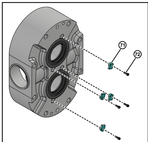
Figure 113 - Remove Screws and Retainer-tab
