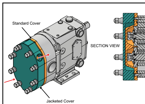
Figure 107 - Jacketed Cover
