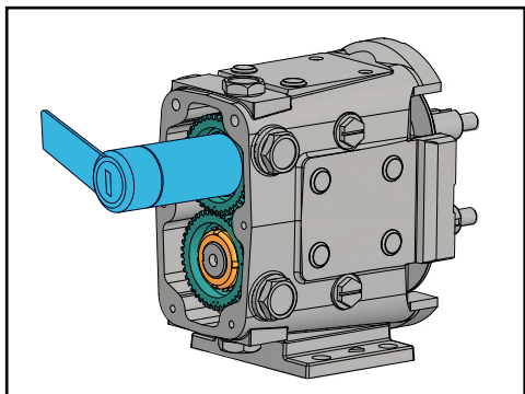
Figure 68 - Install Gear Locknuts
