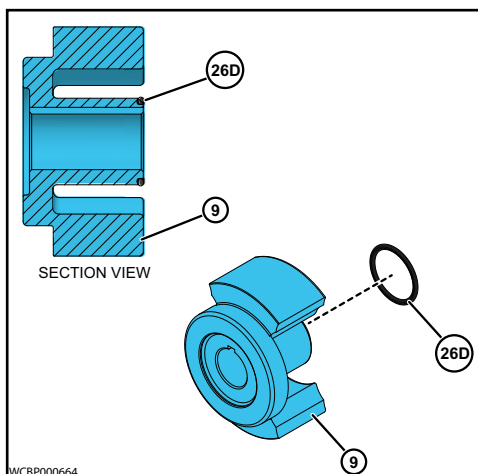
Figure 78 - Install Rotor
