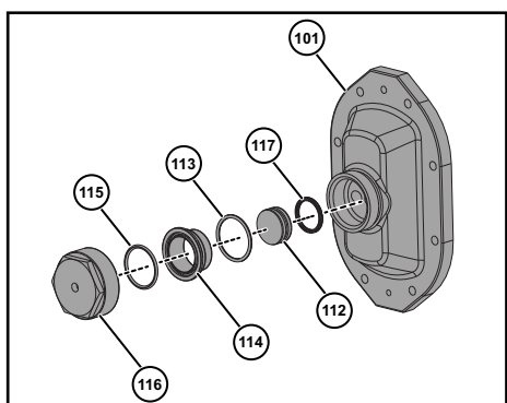
Figure 86 - Pneumatic Piston Cover
