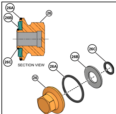
Figure 79 - Rotor Nut Assembly
