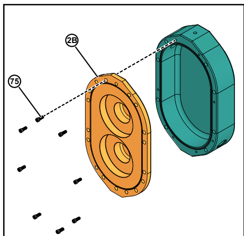
Figure 108 - Remove Cap Screw and Cover
