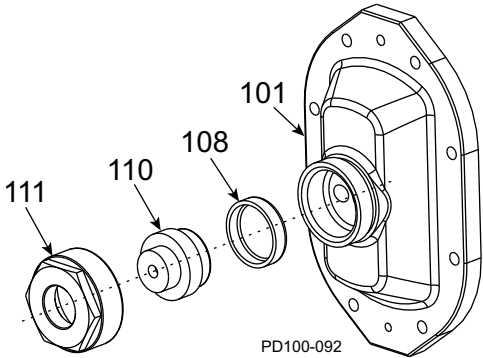
Figure 129 - Pneumatic Diaphragm Vented Cover
