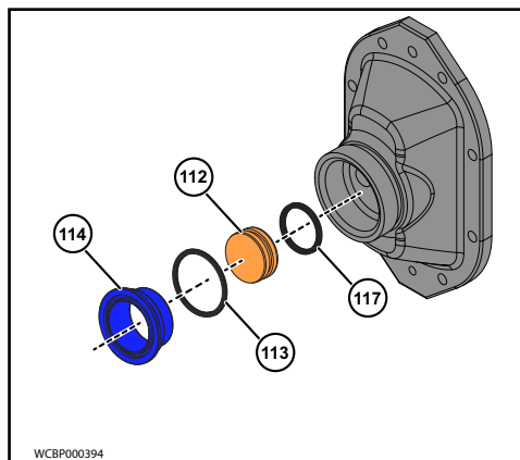
Figure 103 - Install Diaphragm Bushing
