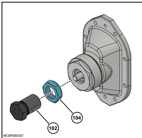
Figure 92 - Install Adjusting Screw
