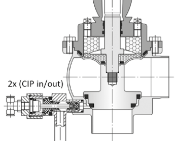
APV DELTA SDMS4
