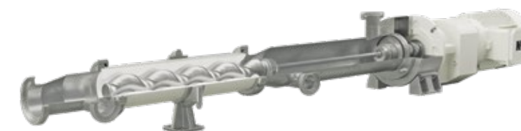
MONO NOV HYGIENIC
