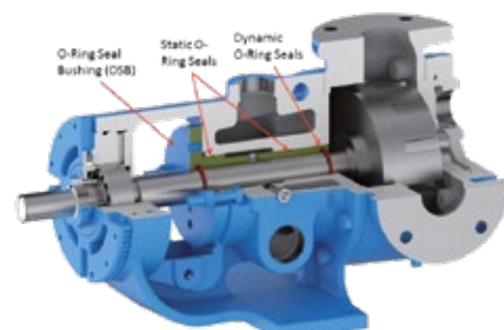
VIKING CHOCOLATE PUMP
