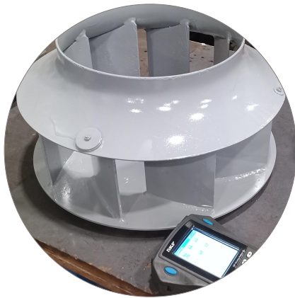
Equilibrage moto-turbine
