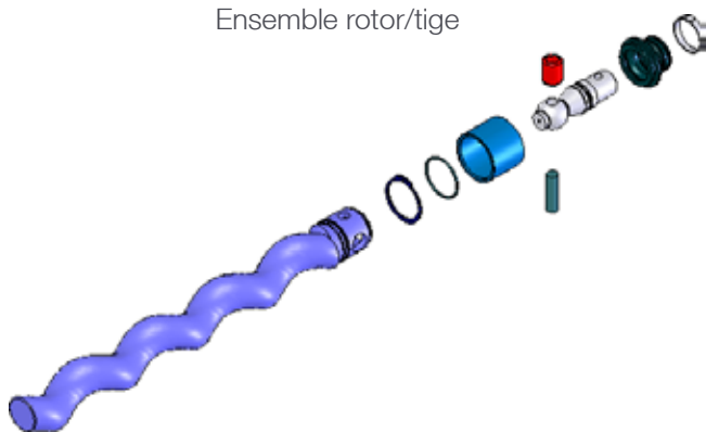
Ensemble rotor/tige
